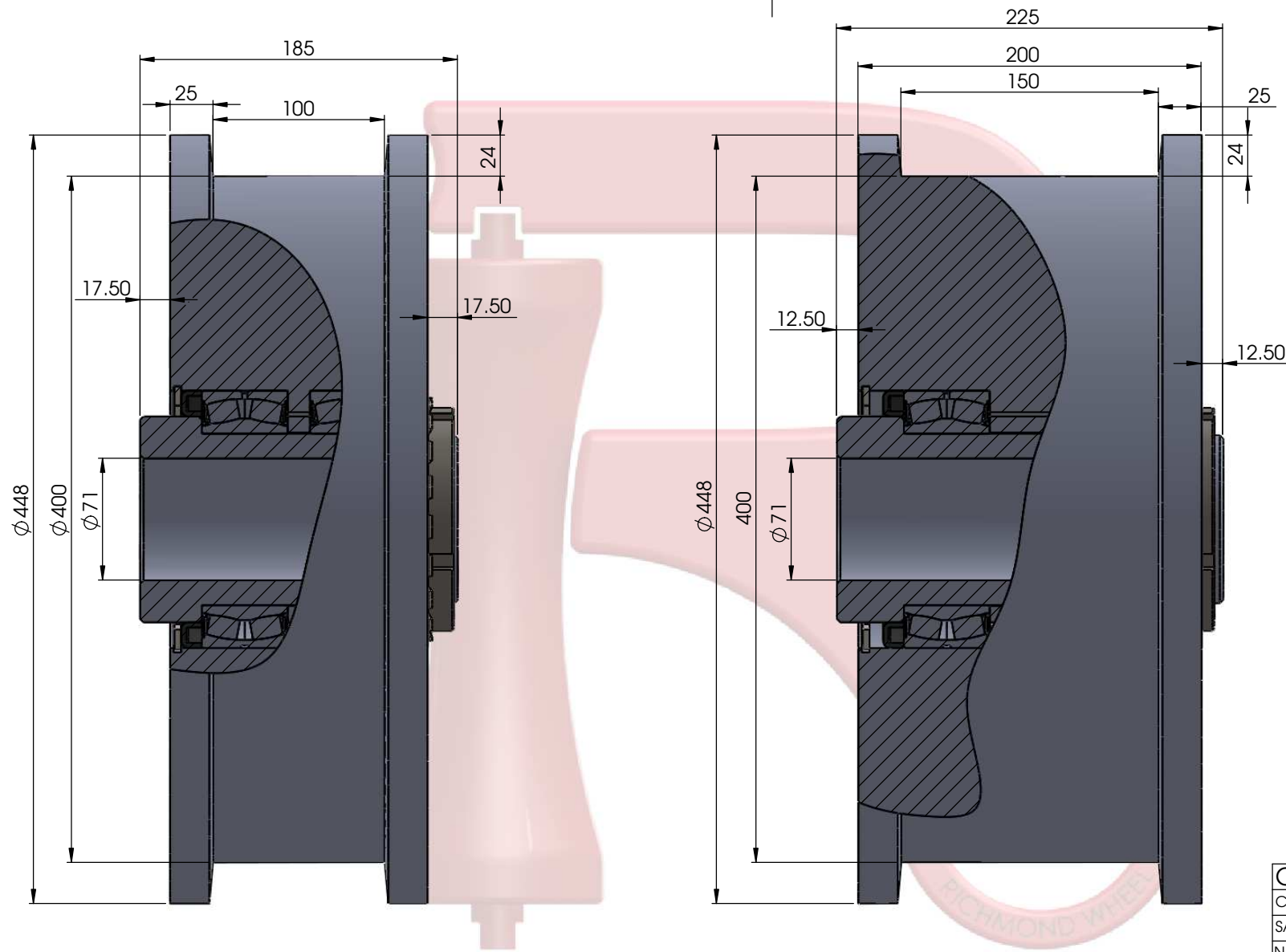
DFST400X100 (100MM SPHERICAL ROLLER BEARINGS TO SUIT M70 PRECISION BOLT)
