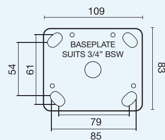
Baseplate Dimensions for Refrigeration Castors
