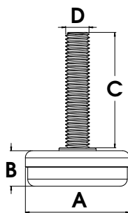
FIXED - STEEL/NYLON FOOT LFR361045FSN
